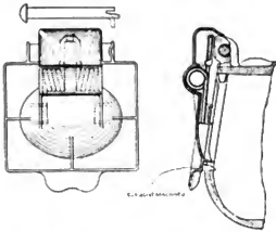
Figs. 4490-4491. Symington M. C. B. Journal Box Lid with Torsion Spring.
